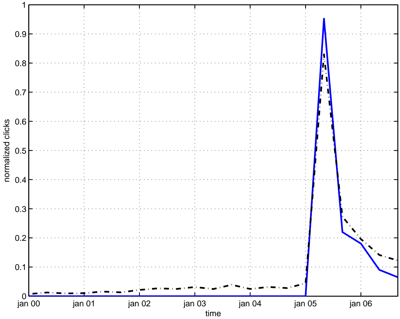
u(4) group theory
