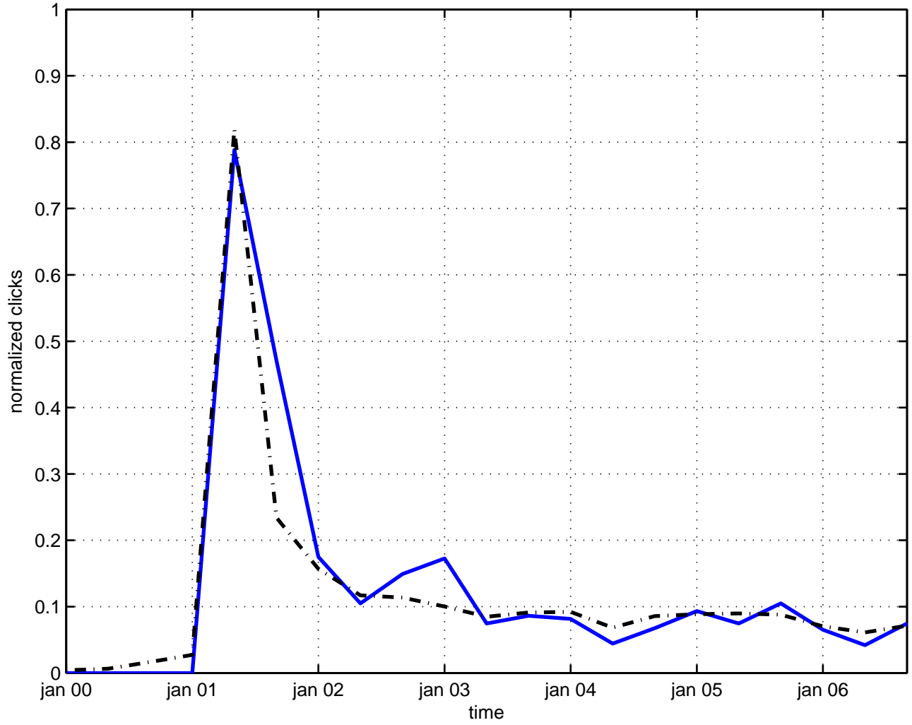
u(3) x u(3) gauge field theory
