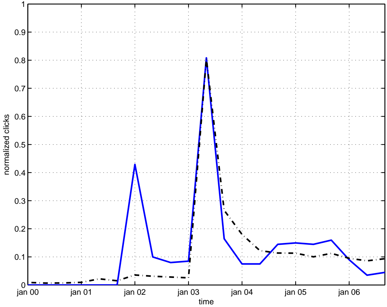
u(2) transformation
