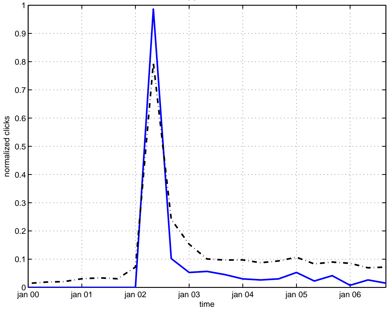
u(2) instanton
