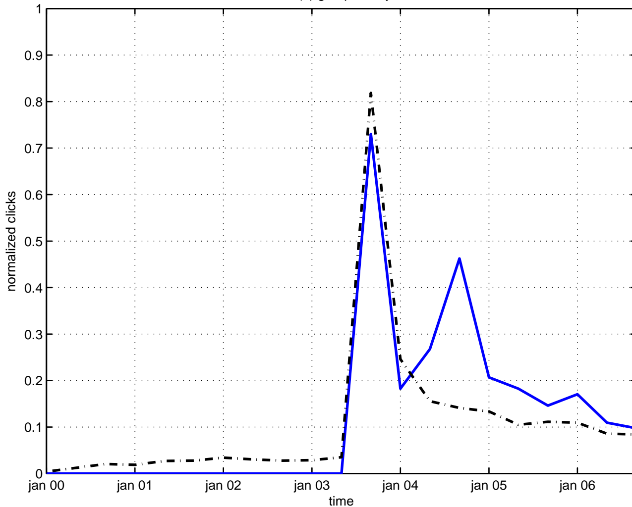
u(2) group theory
