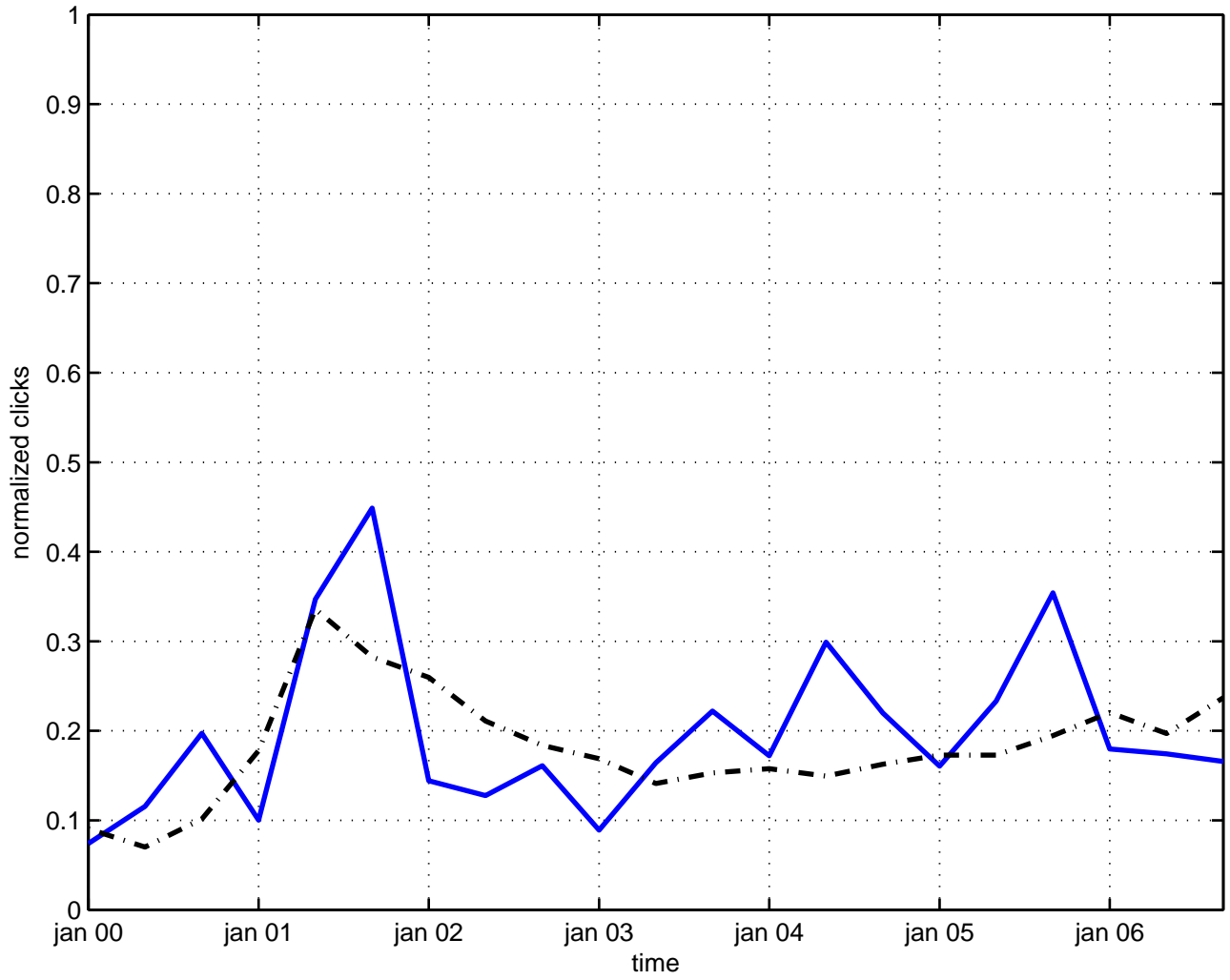
u(2) gauge field theory
