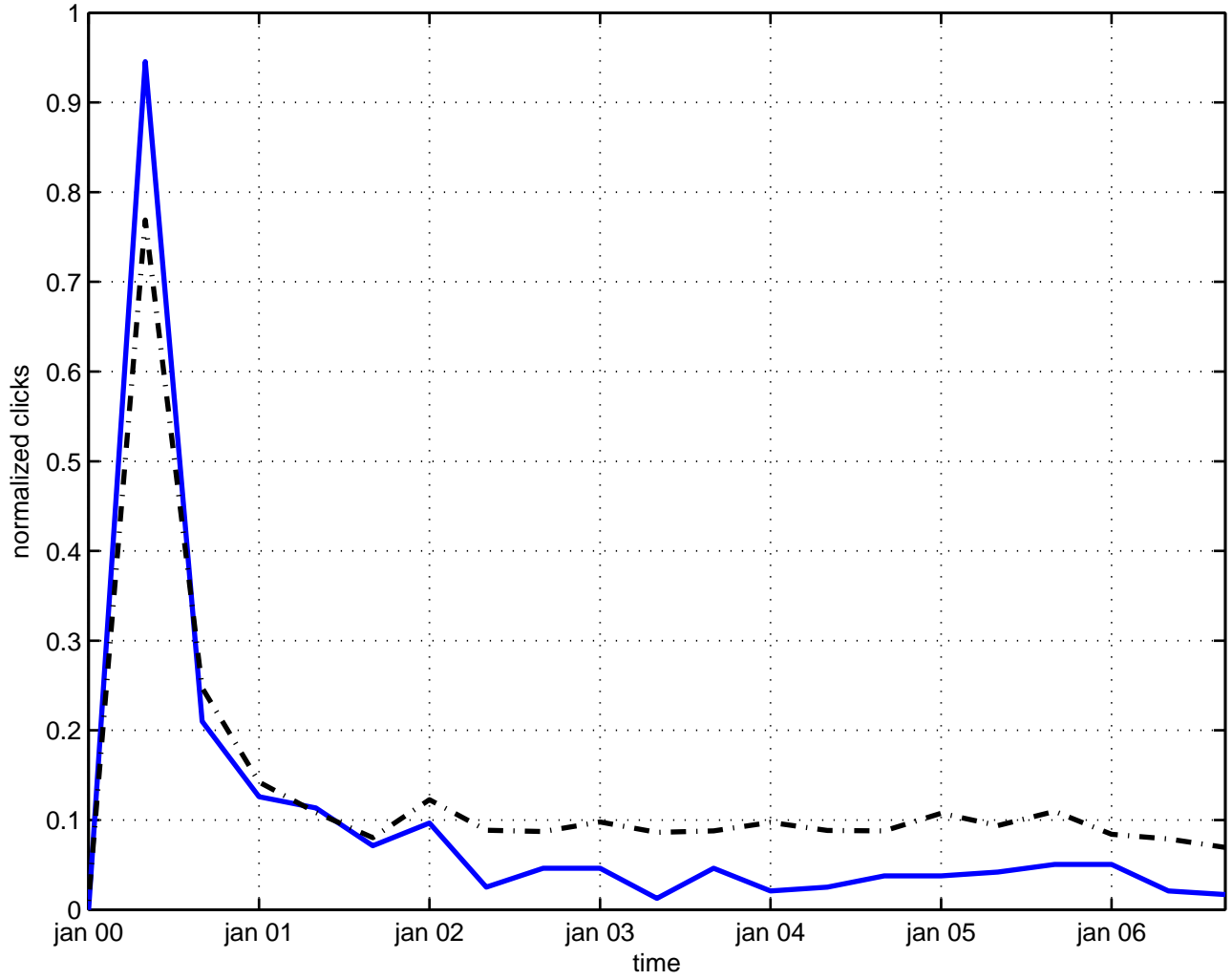
u(1,n) gauge field theory
