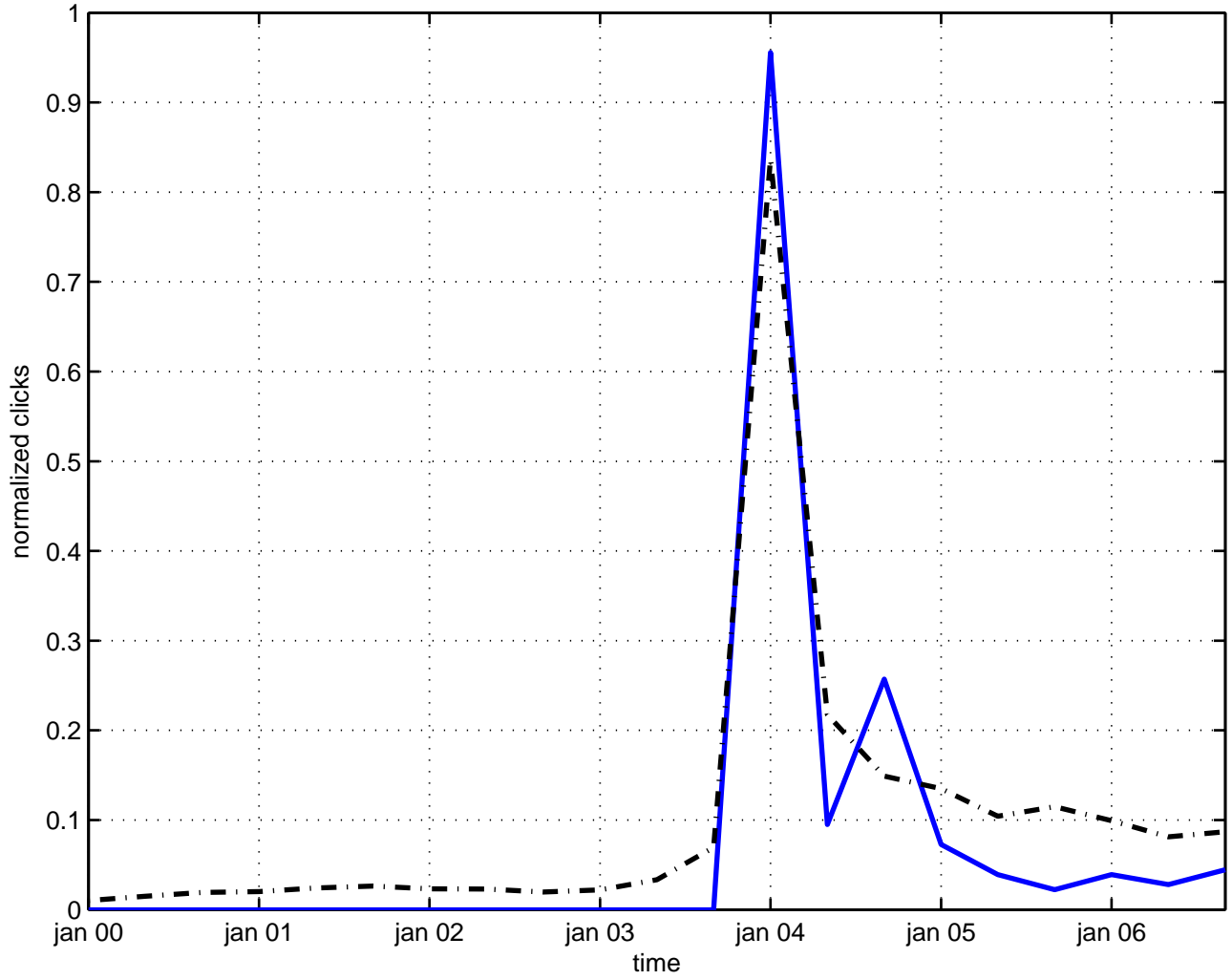
u(1,3) gauge field theory
