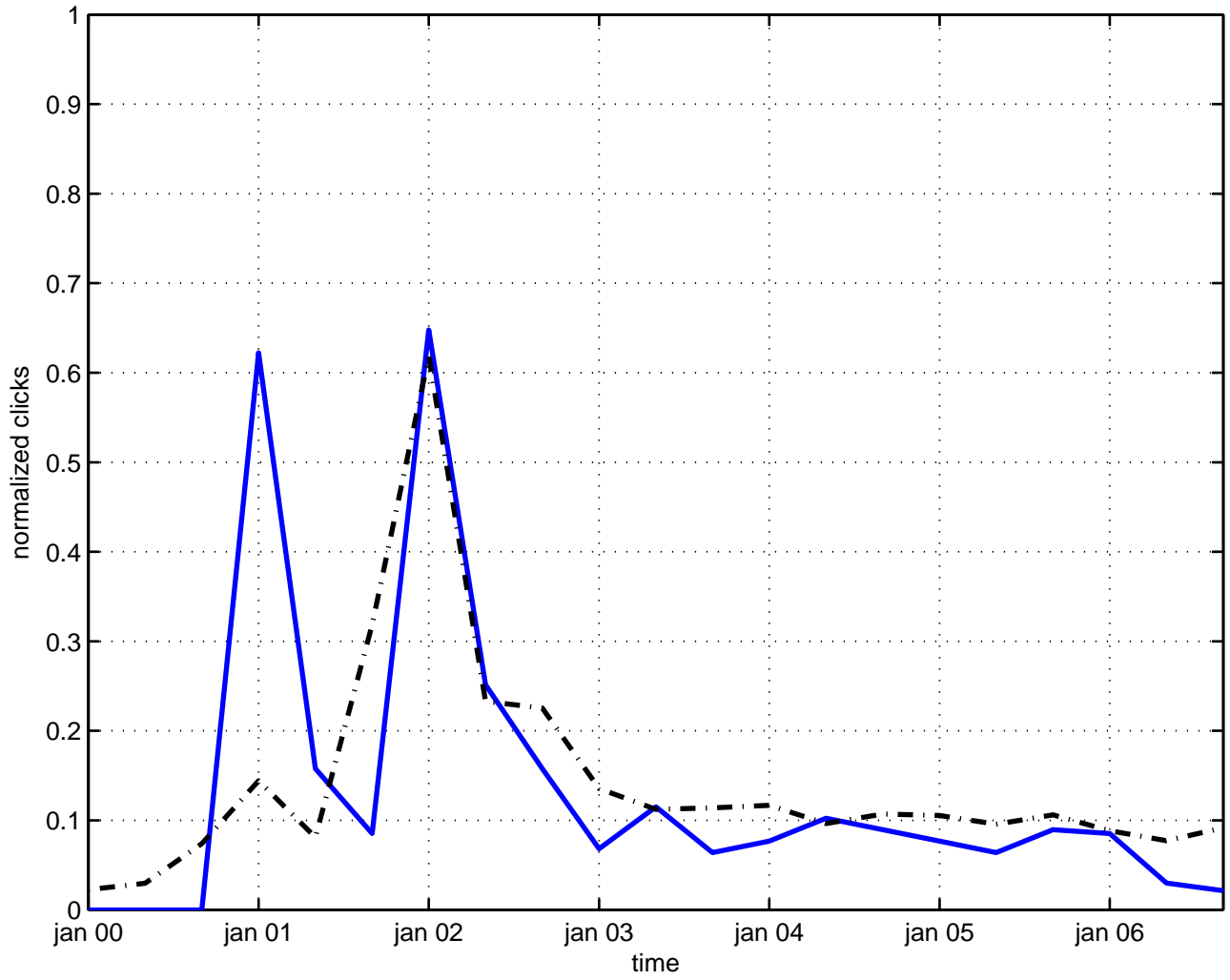
u(1,1) symmetry
