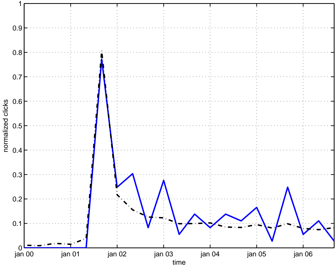
u(1,1) group theory
