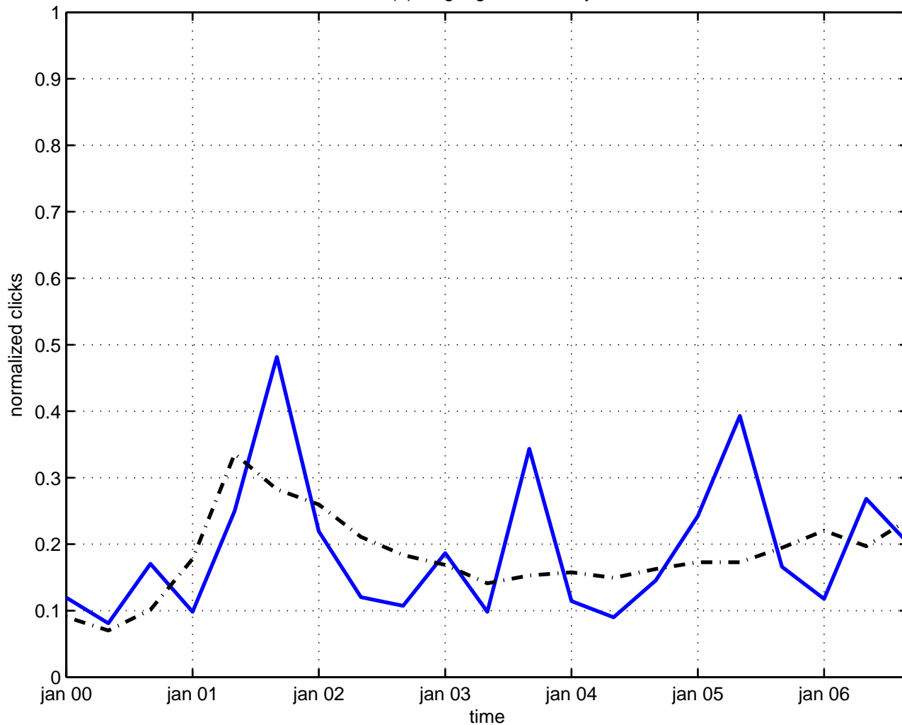
u(1)**n gauge field theory
