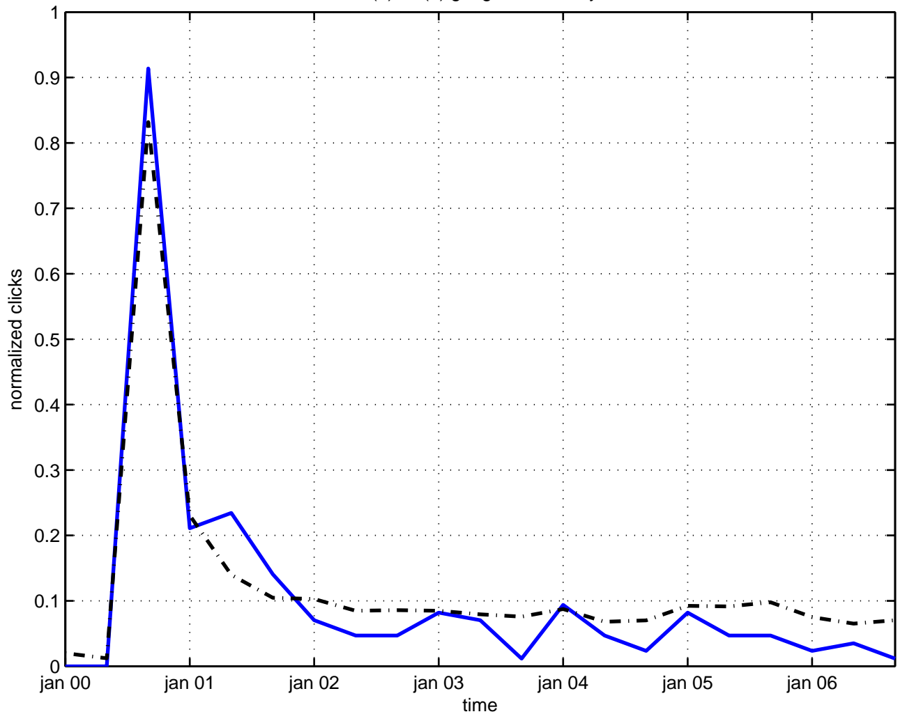
u(1) x z(2) gauge field theory
