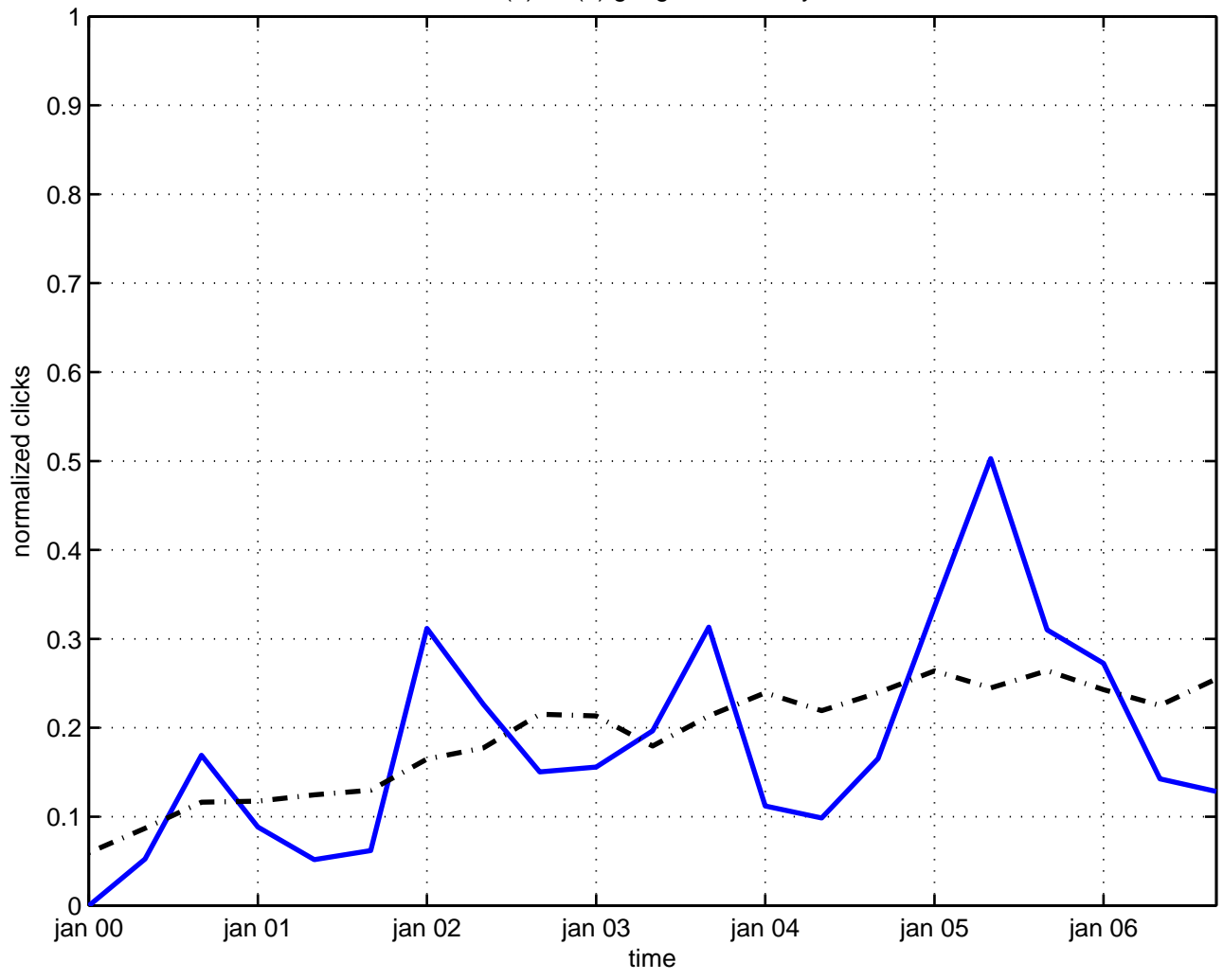
u(1) x u(1) gauge field theory
