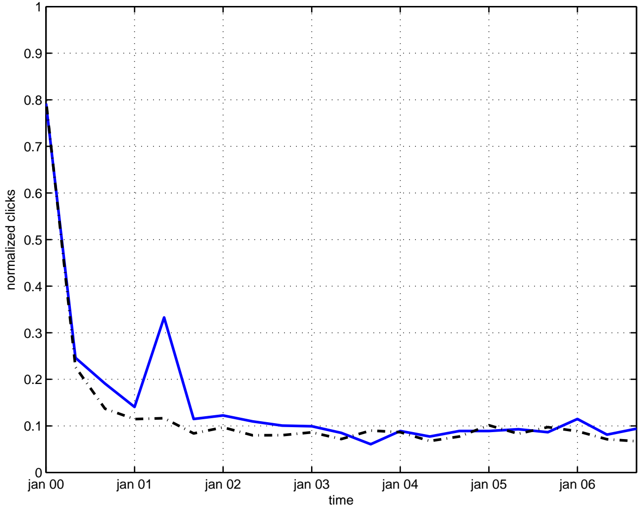
u(1) transformation
