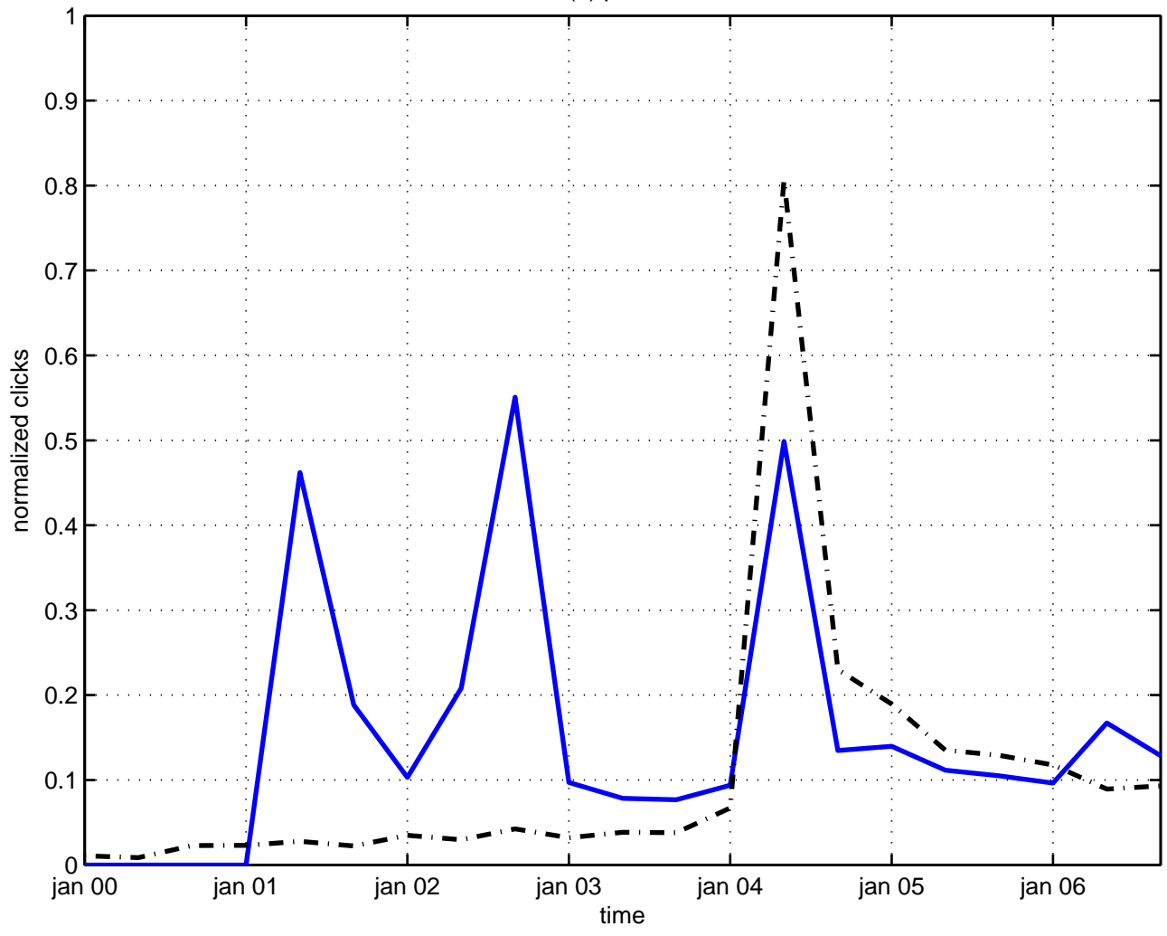
u(1) problem
