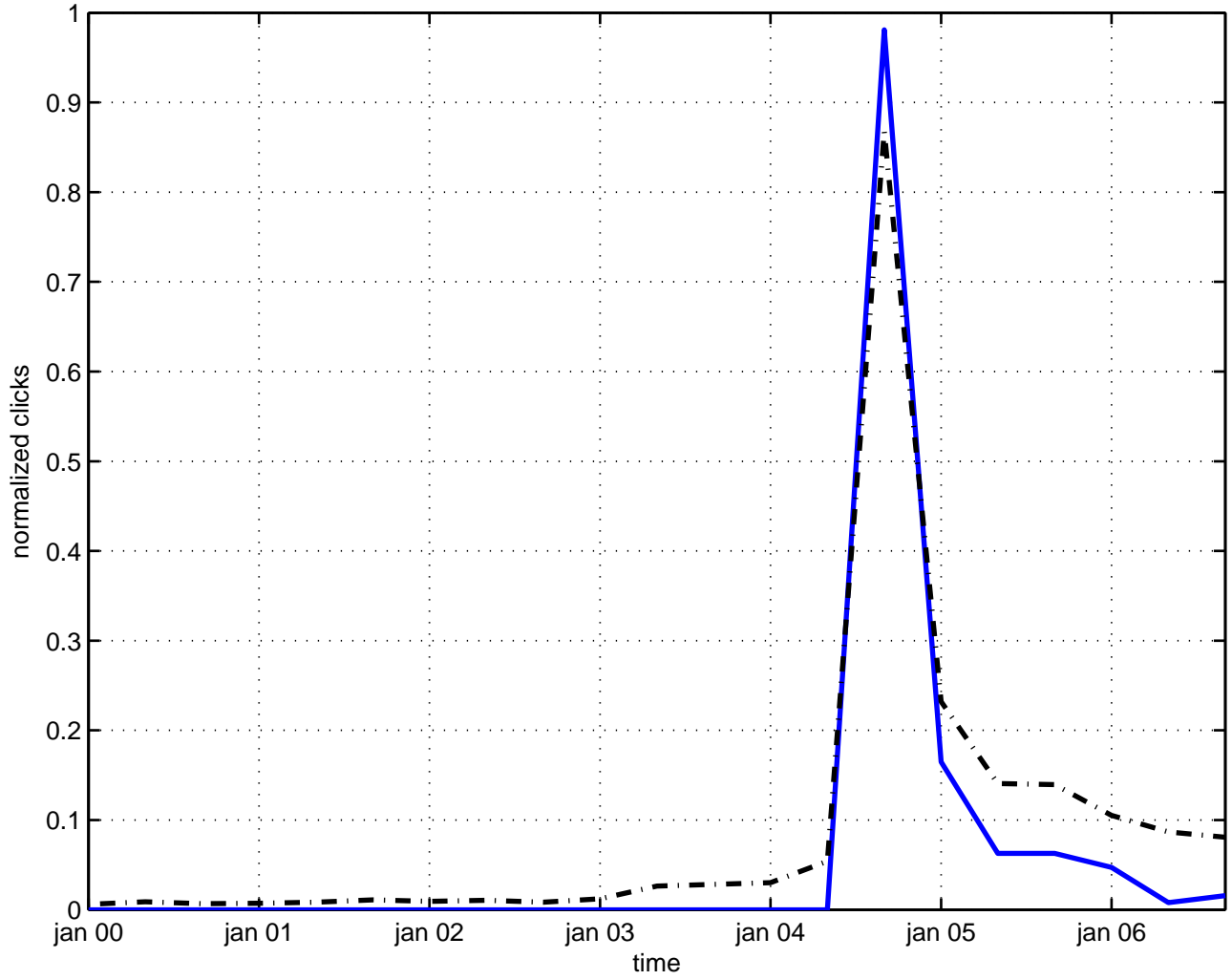
u(1) isometry
