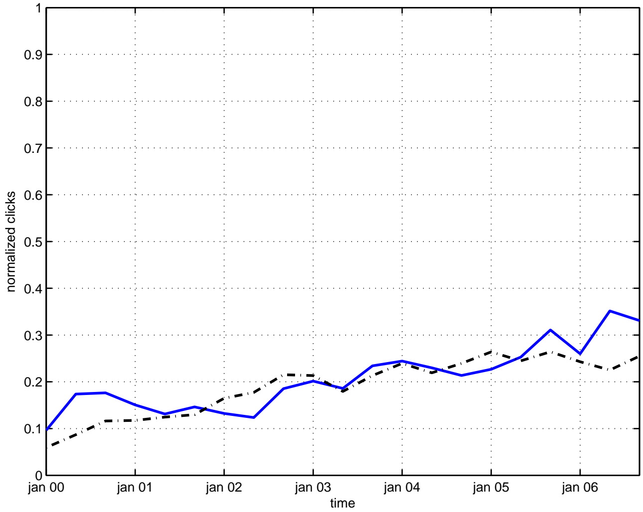
u(1) gauge field theory
