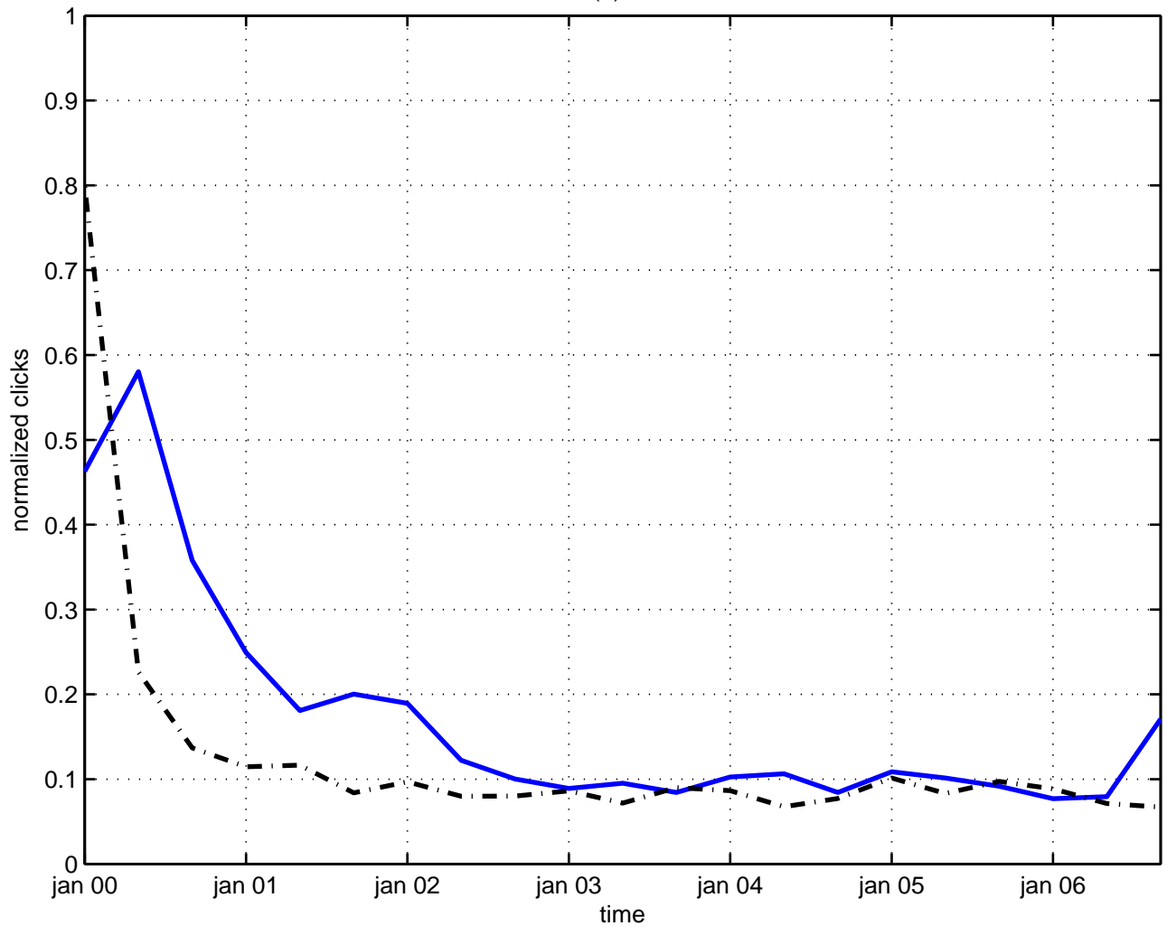
u(1) flux
