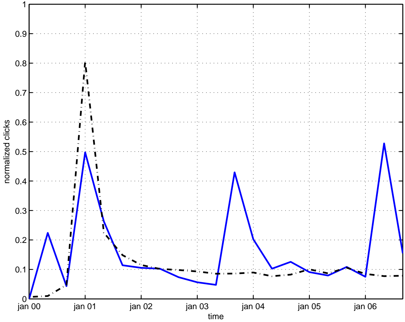
u(1) fibre bundle
