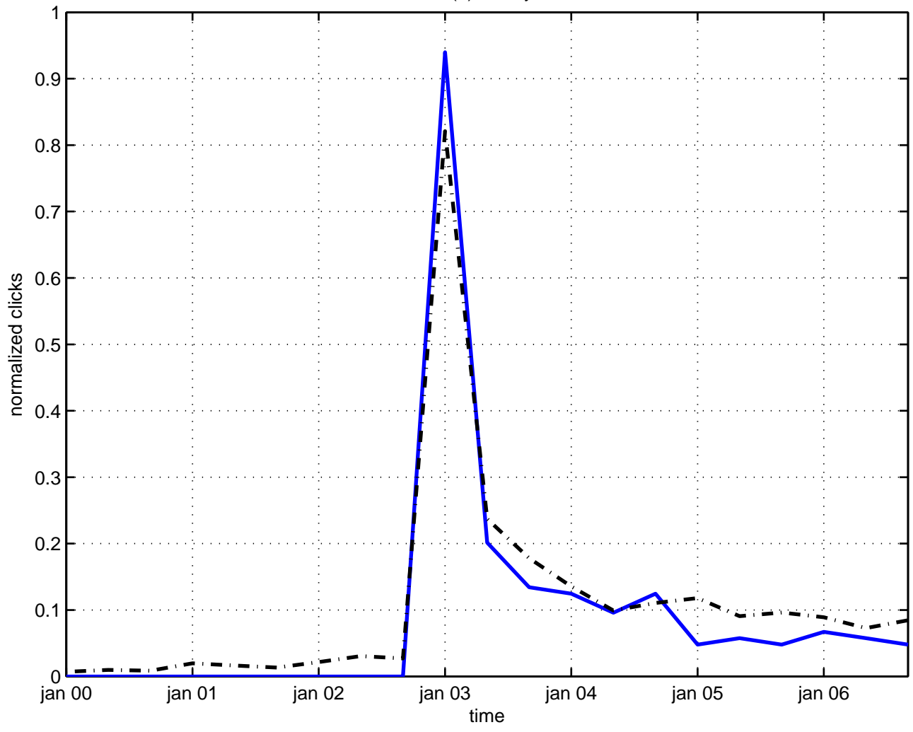
u(1) duality
