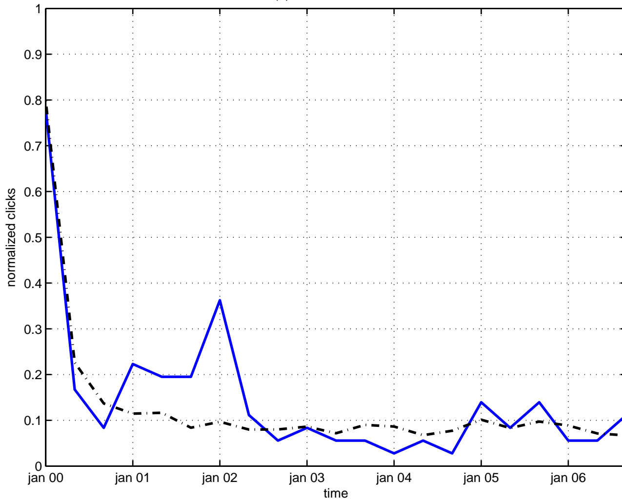
u(1) chern-simons term
