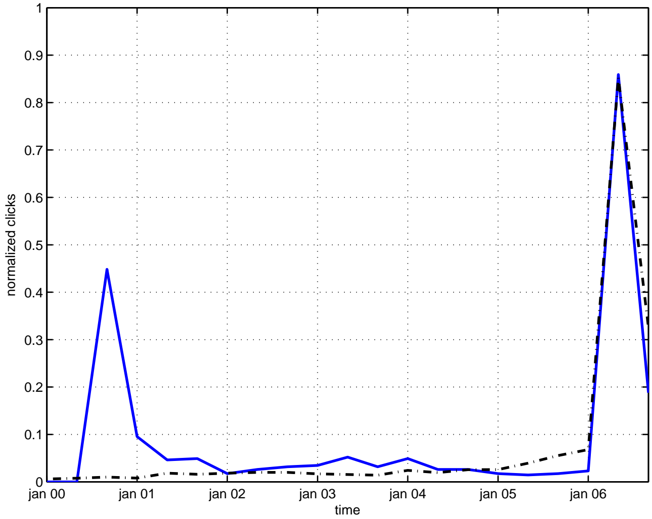
two-point function graviton
