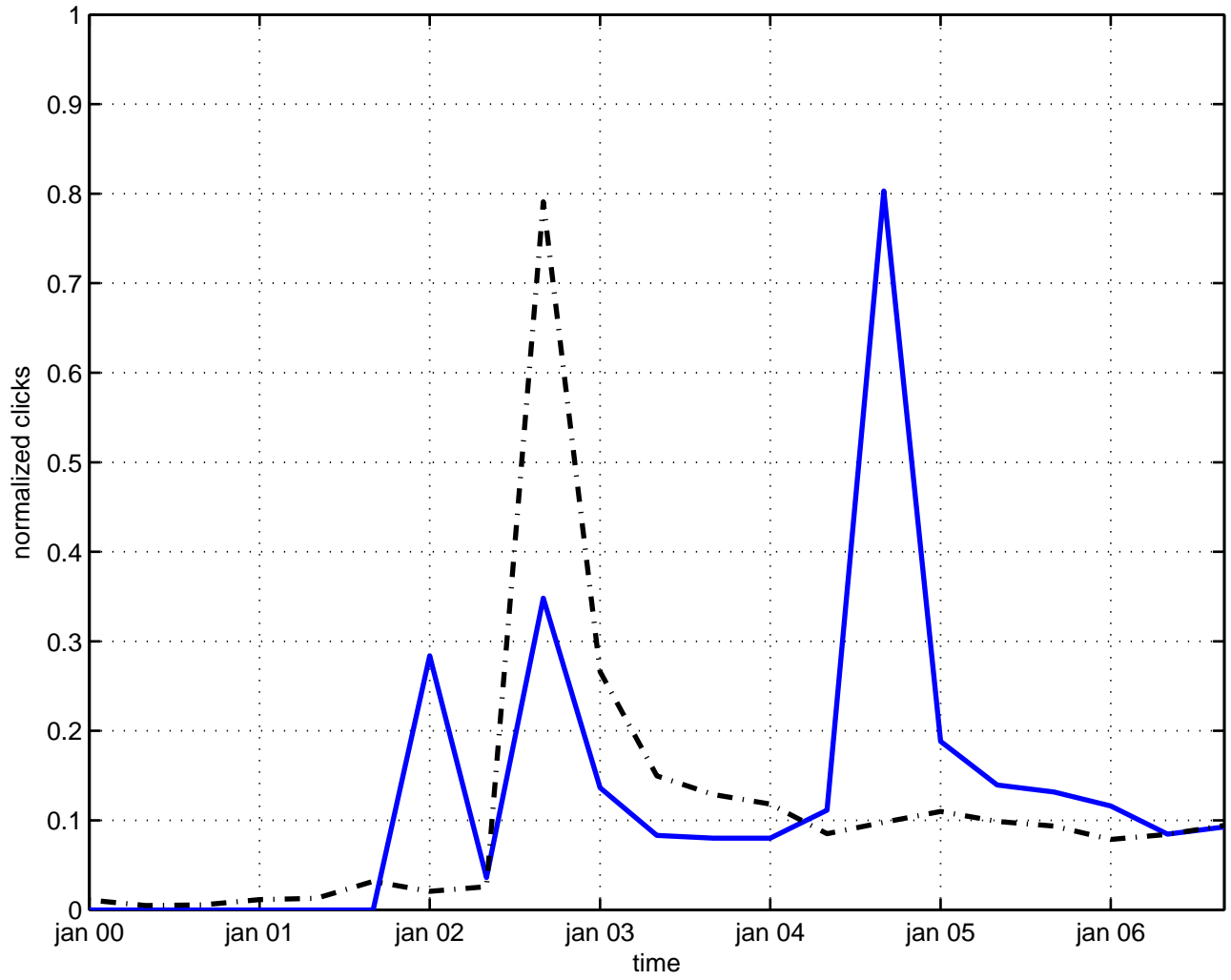
two-particle scattering
