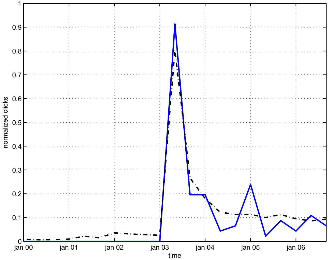
two-particle model
