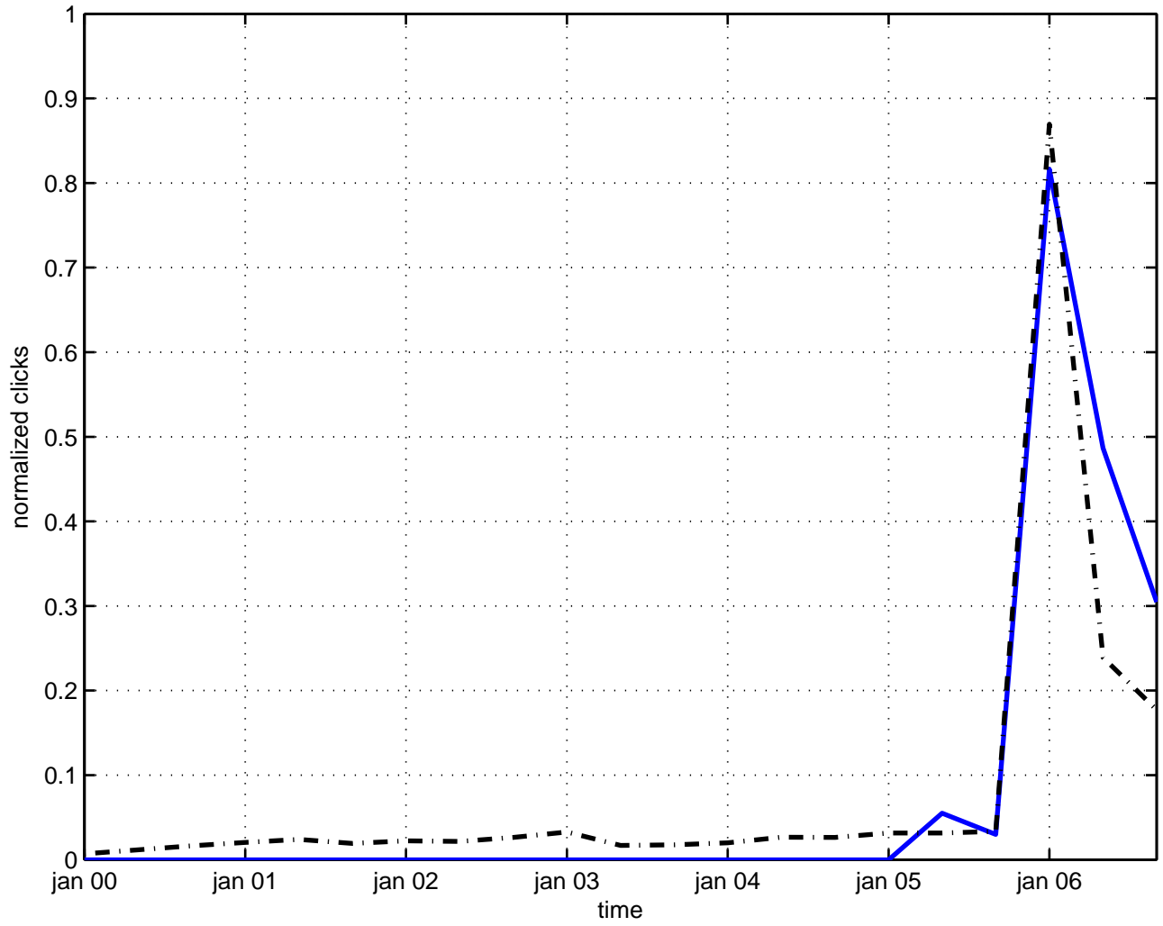
twist symmetry
