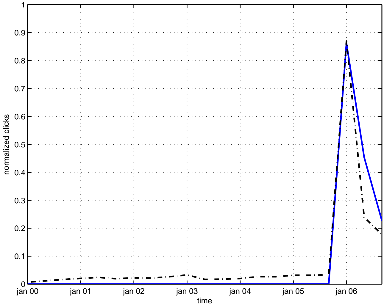
twist quantization
