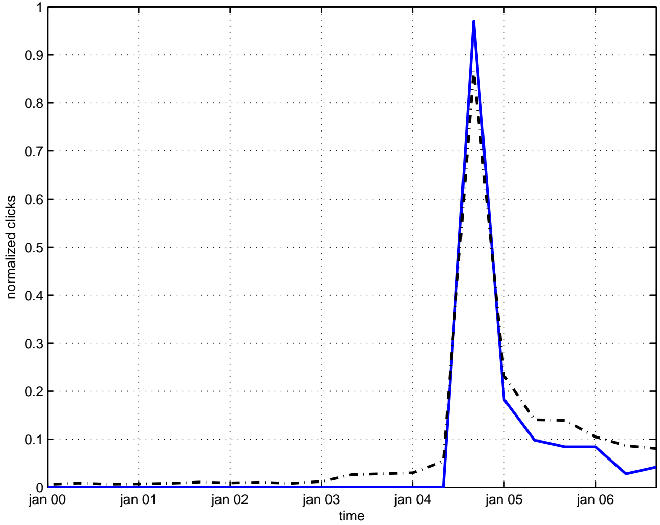
twist multiplet
