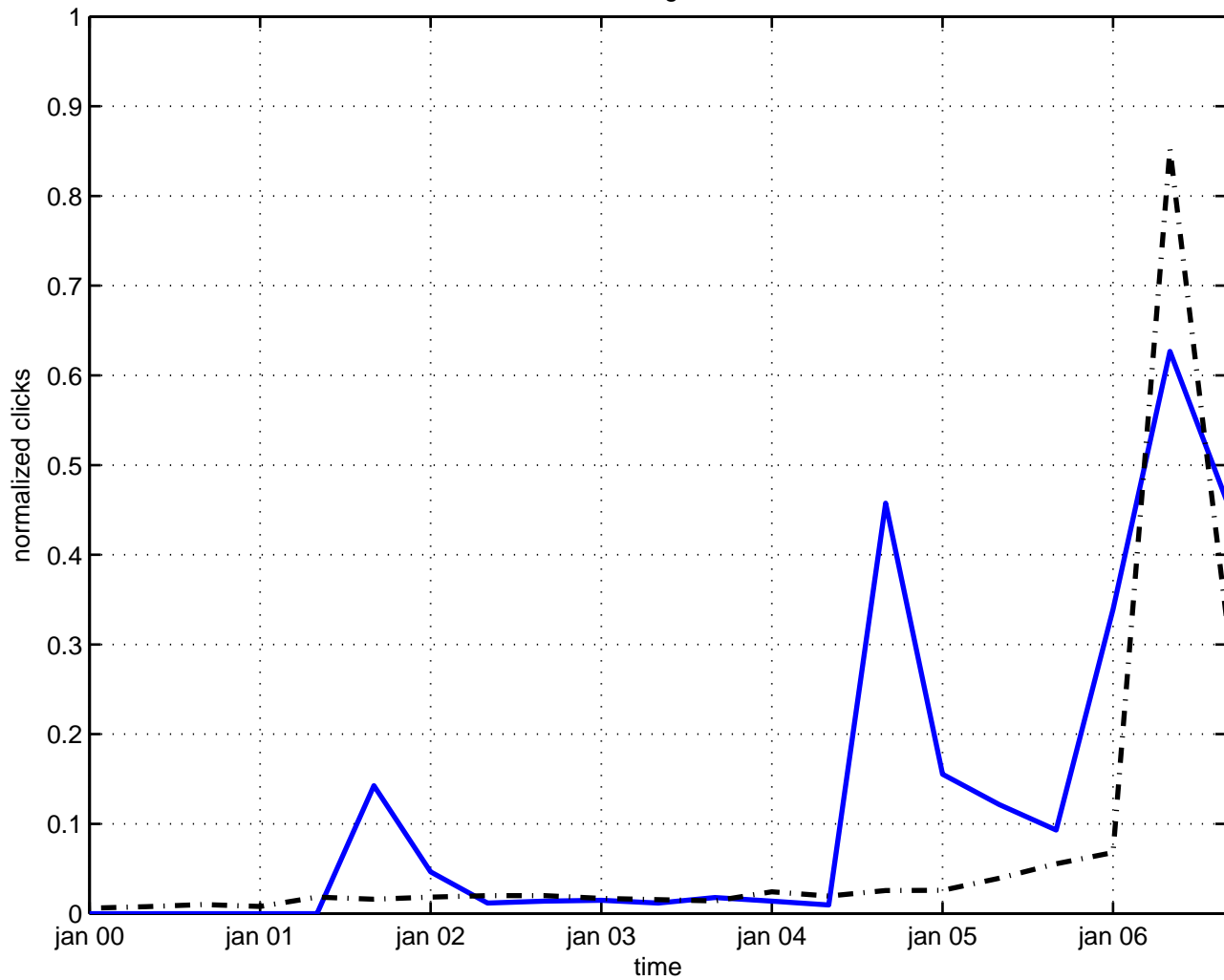
twist algebra
