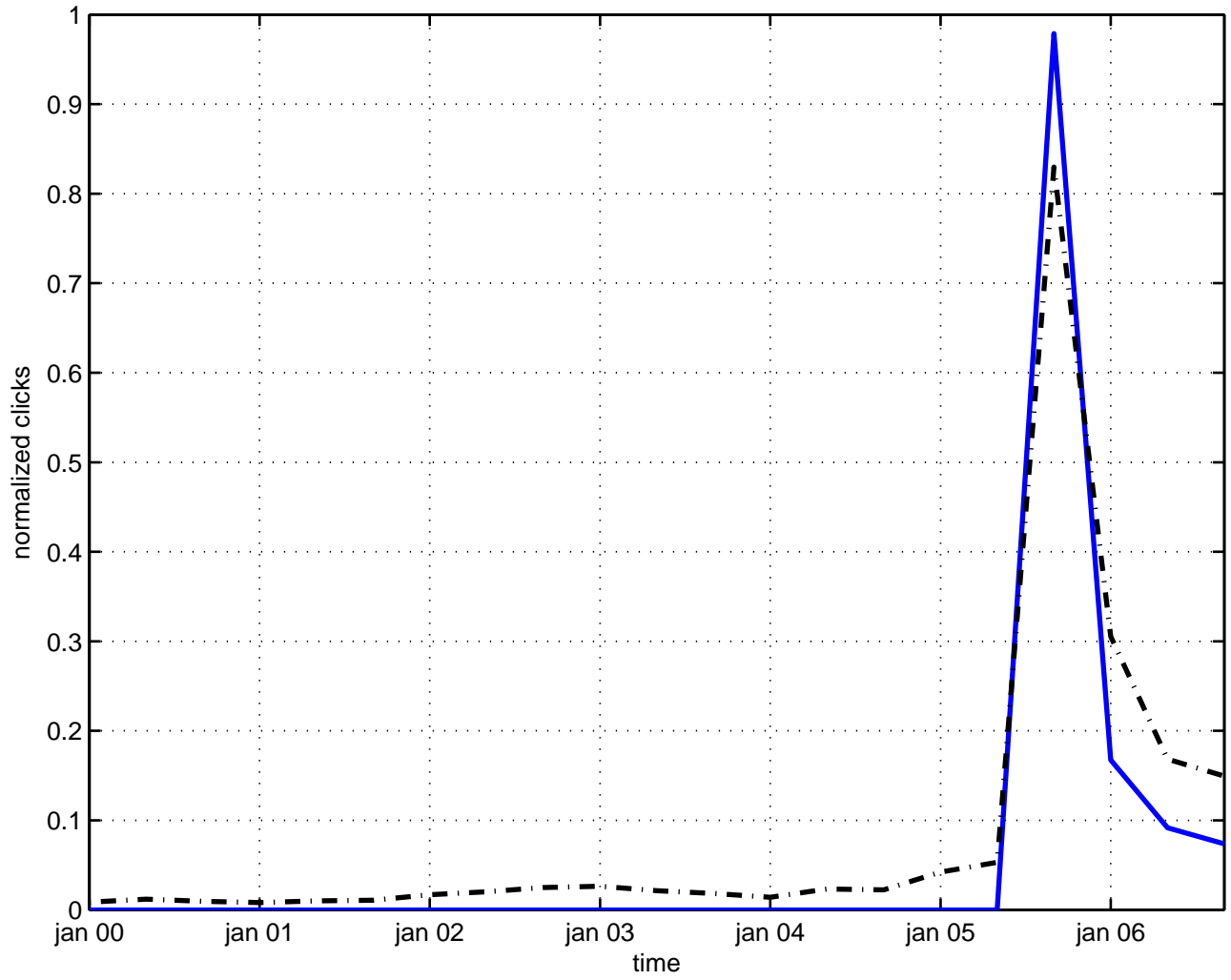
tunneling vacuum state
