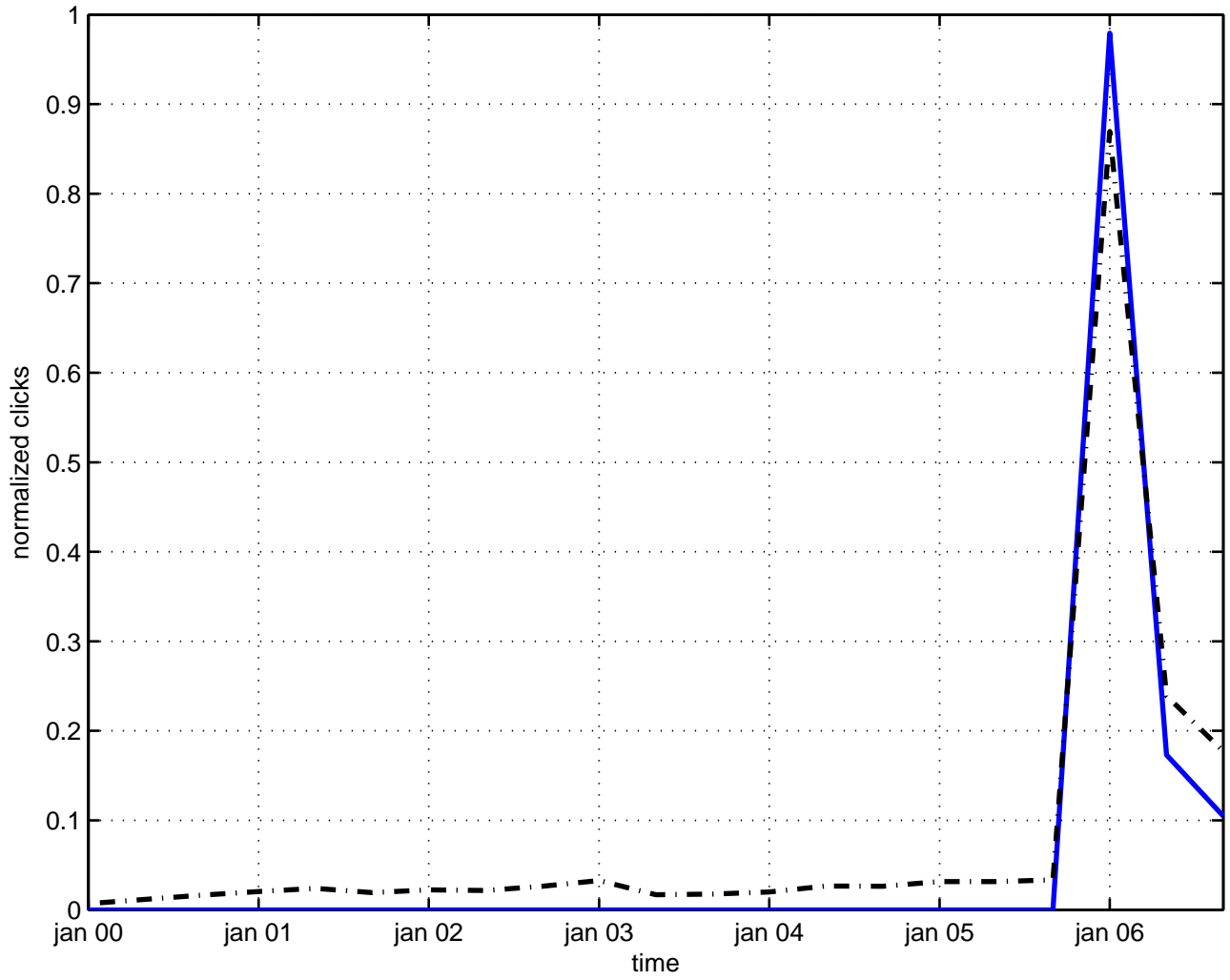
tsallis statistics
