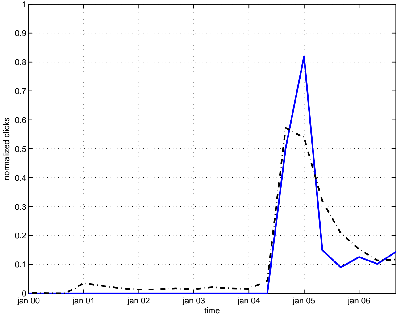
truth quark
