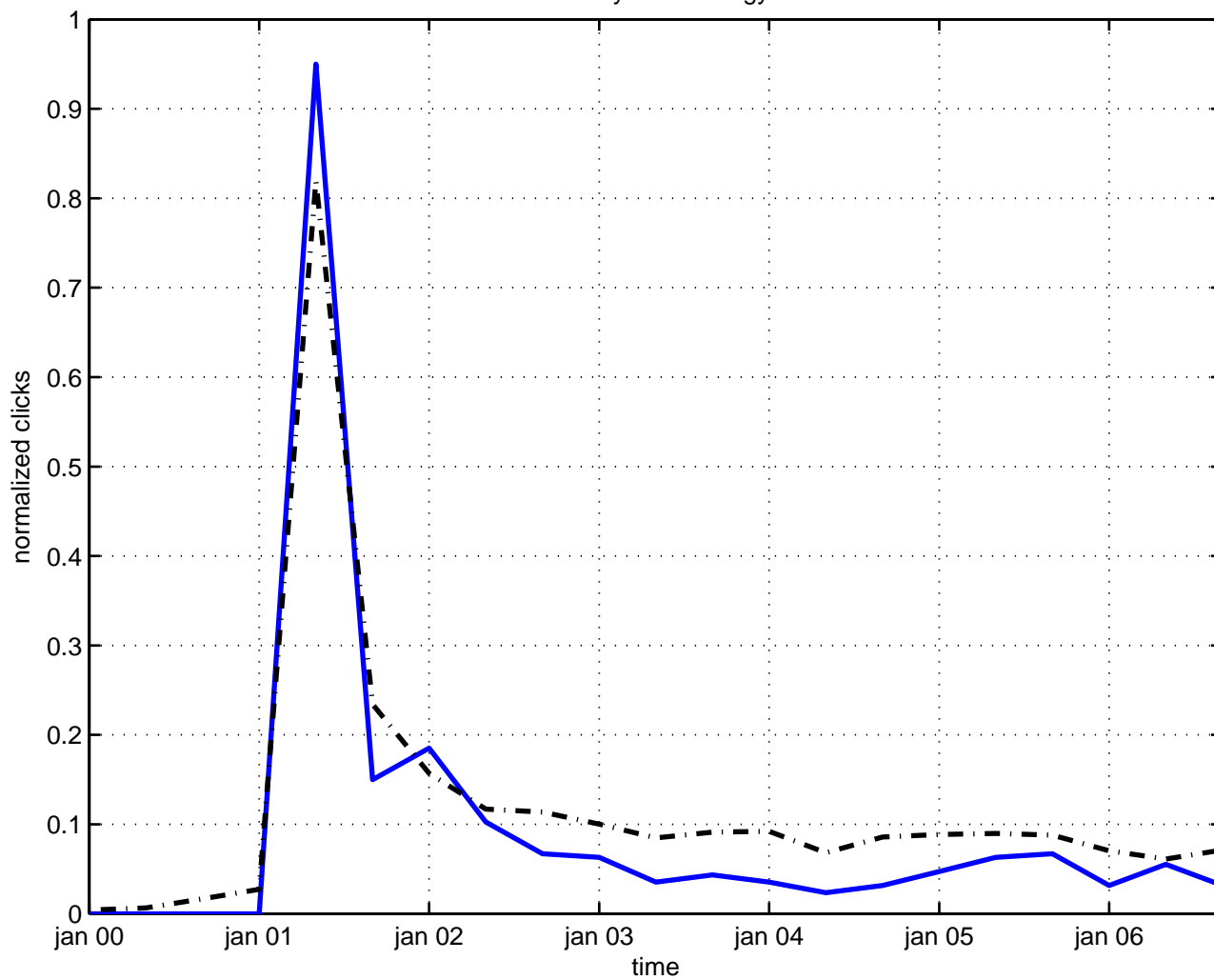
triviality cohomology
