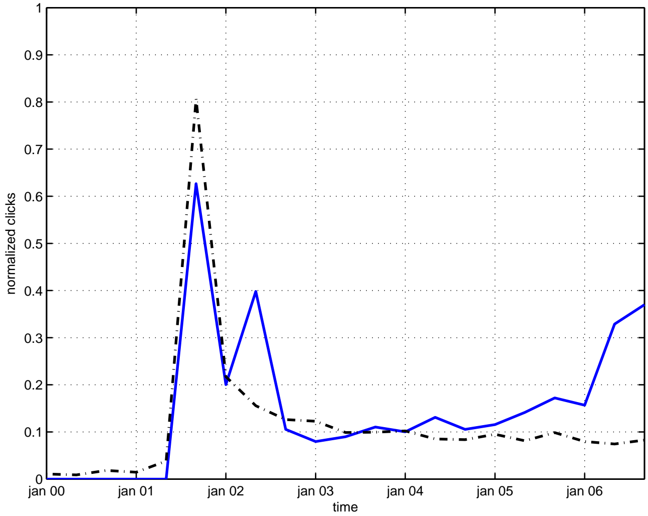
triplet algebra
