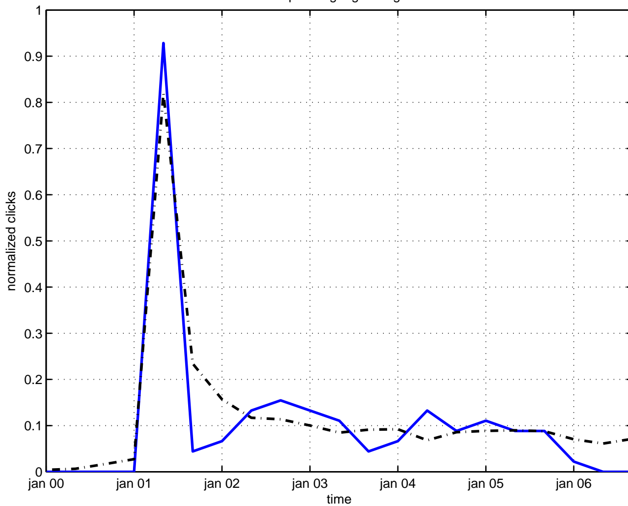
triplectic gauge fixing
