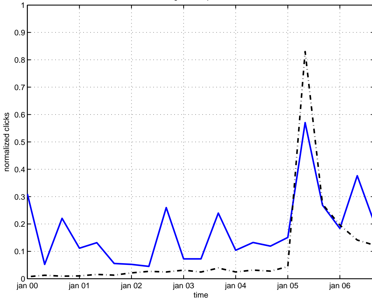
triangulation space-time
