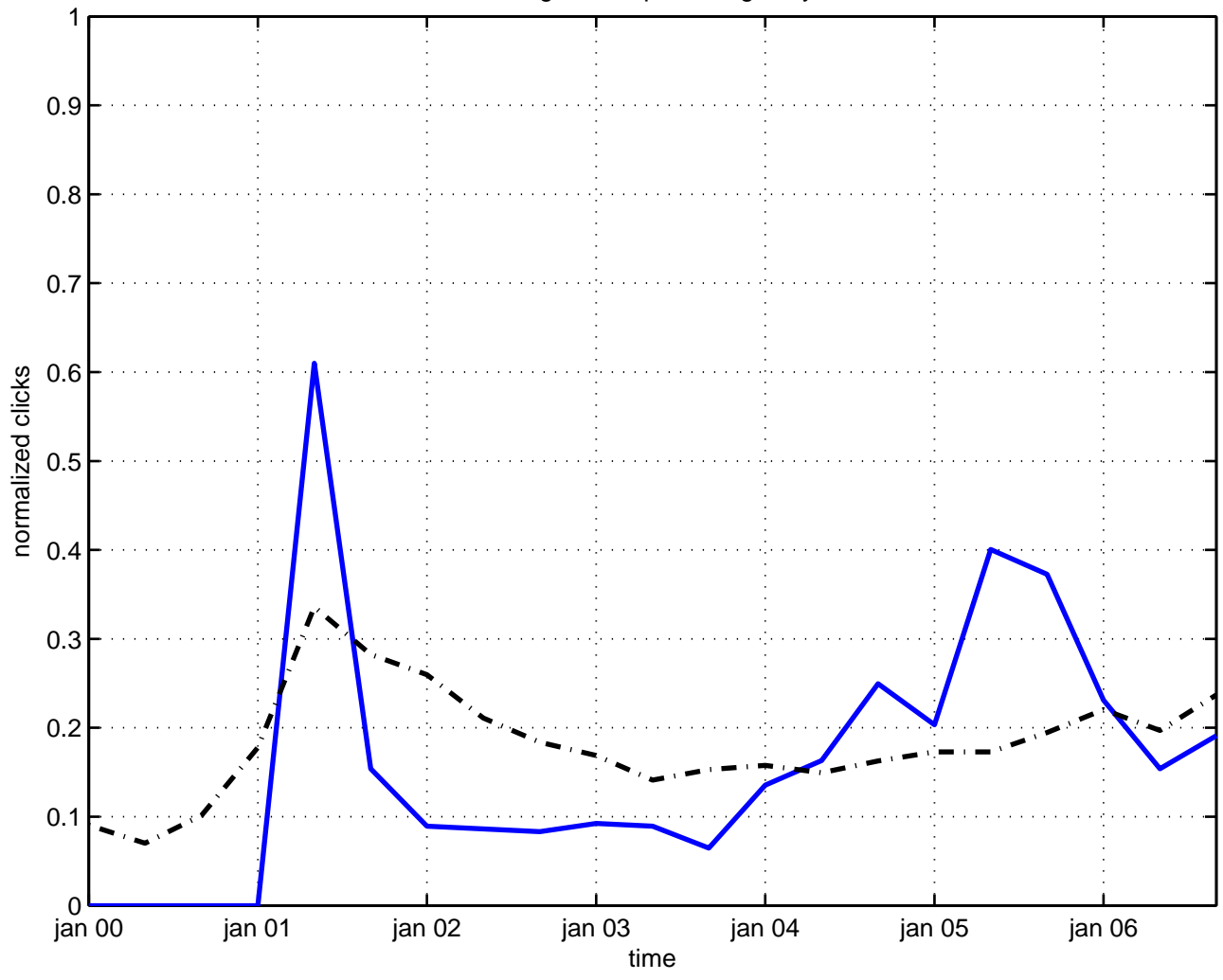
triangulation quantum gravity
