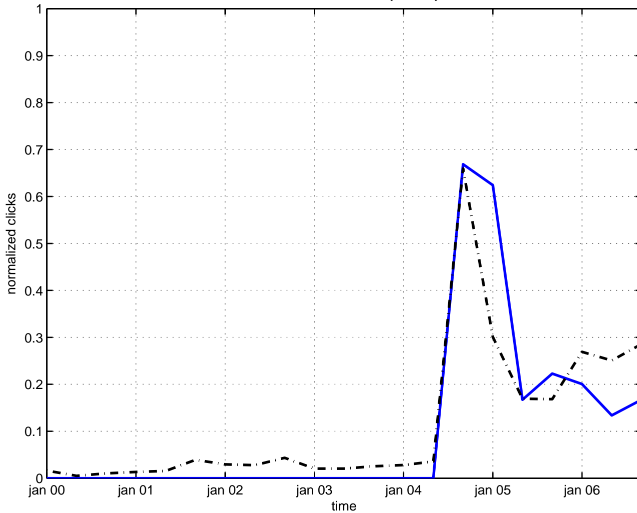
transverse momentum symmetry
