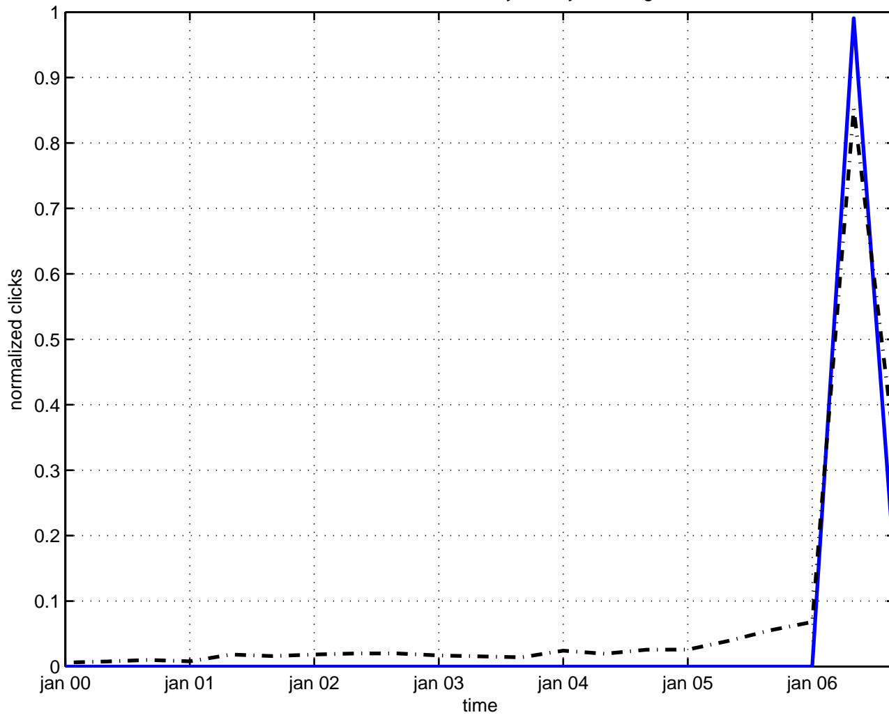
transverse momentum symmetry breaking
