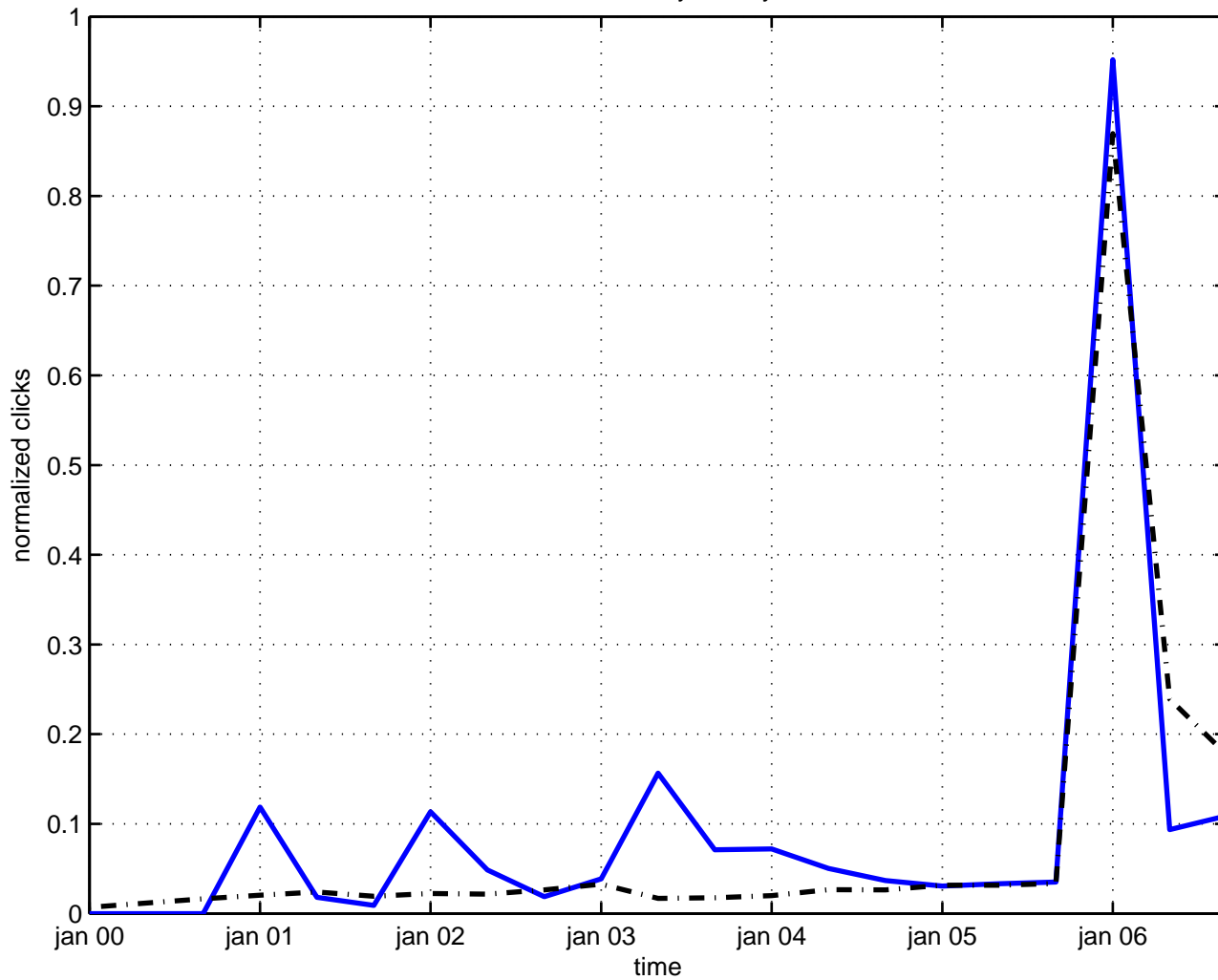
translation symmetry
