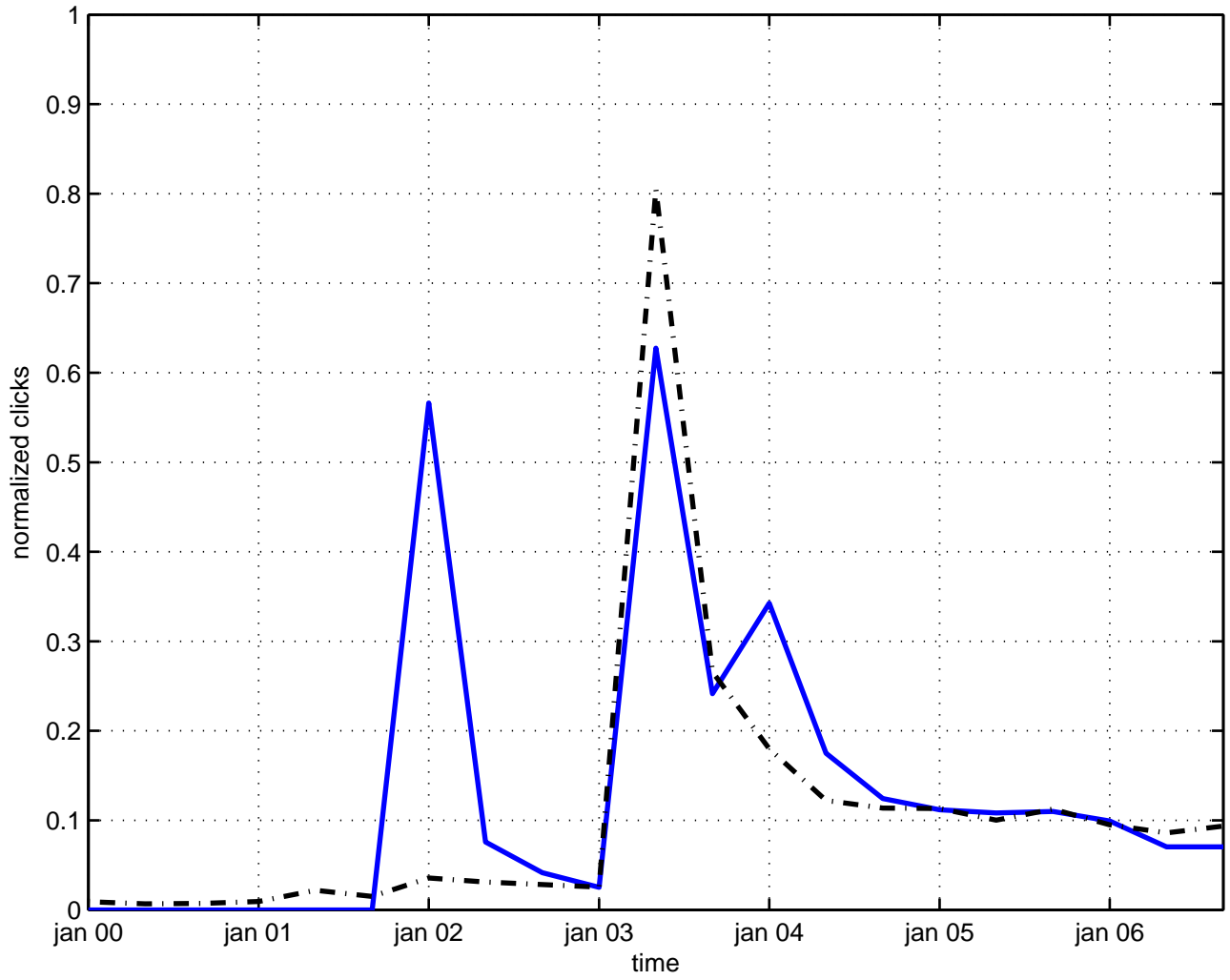
transition instanton
