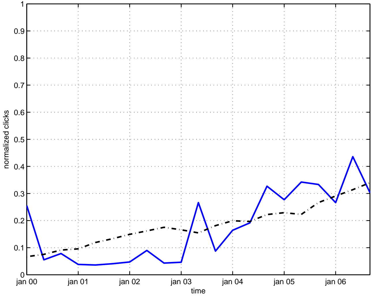
transformation symmetry
