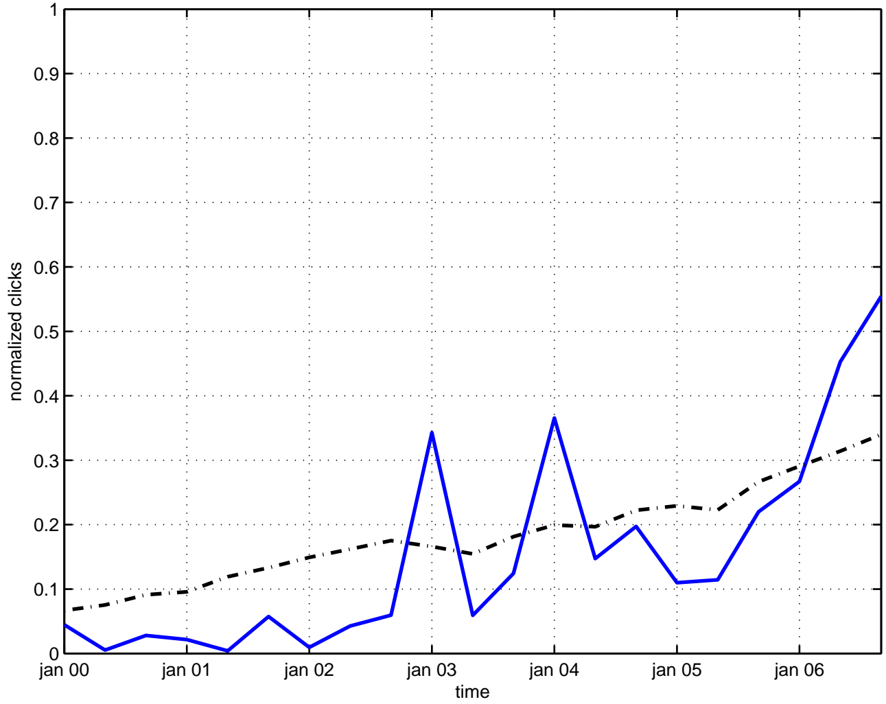
transformation space-time
