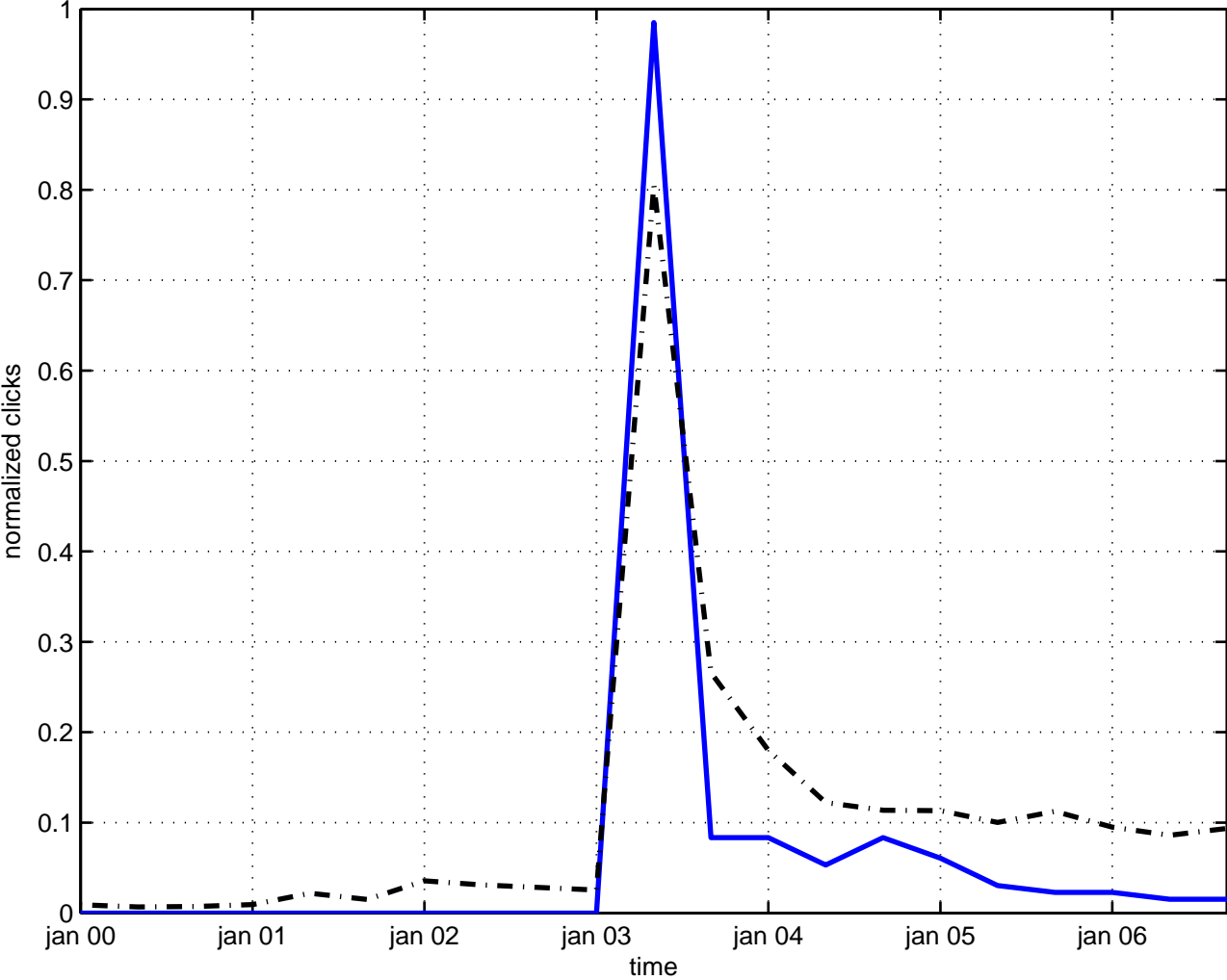
transformation renormalization
