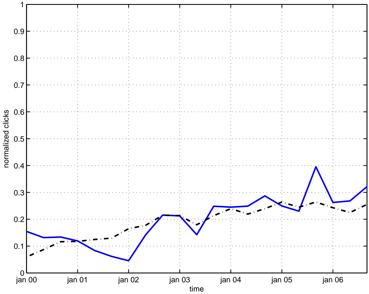
transformation renormalization group
