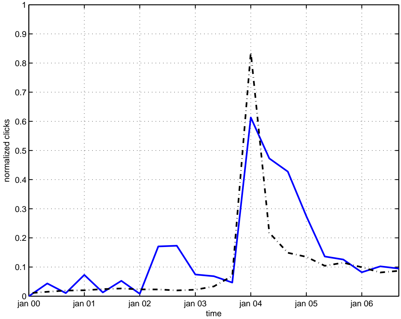
transformation parity
