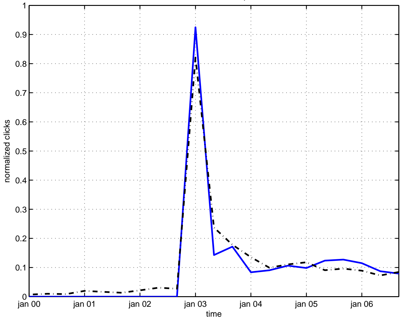
transformation multiplet
