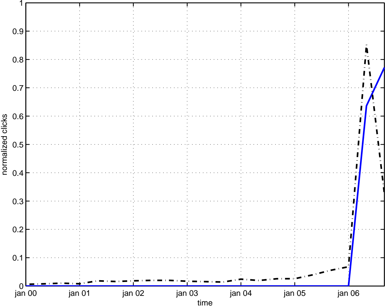
trajectory dynamical system
