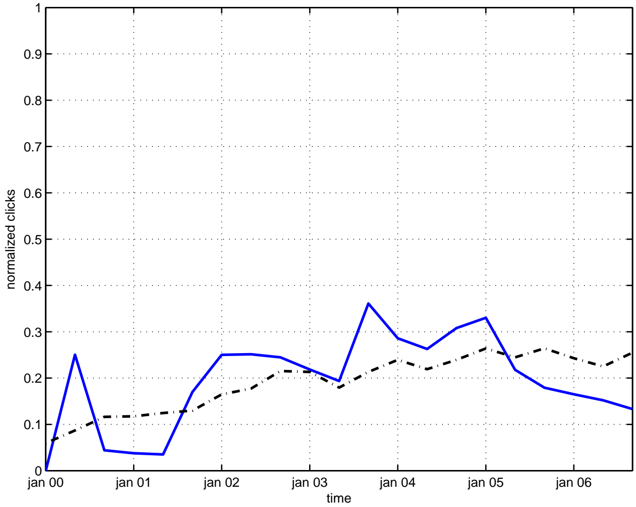
torus m-theory
