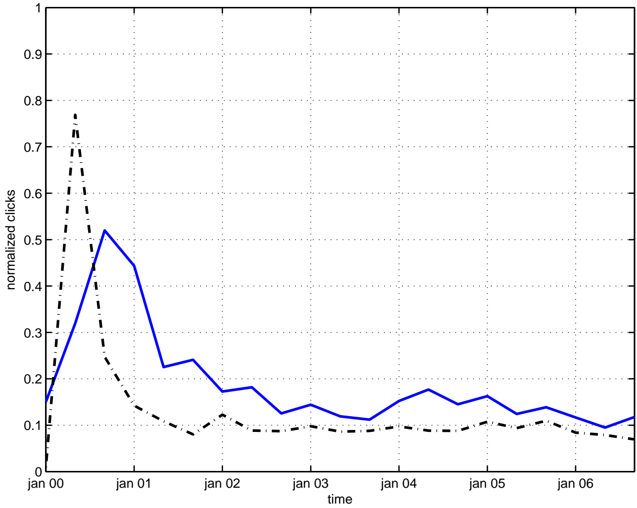
torus field theory
