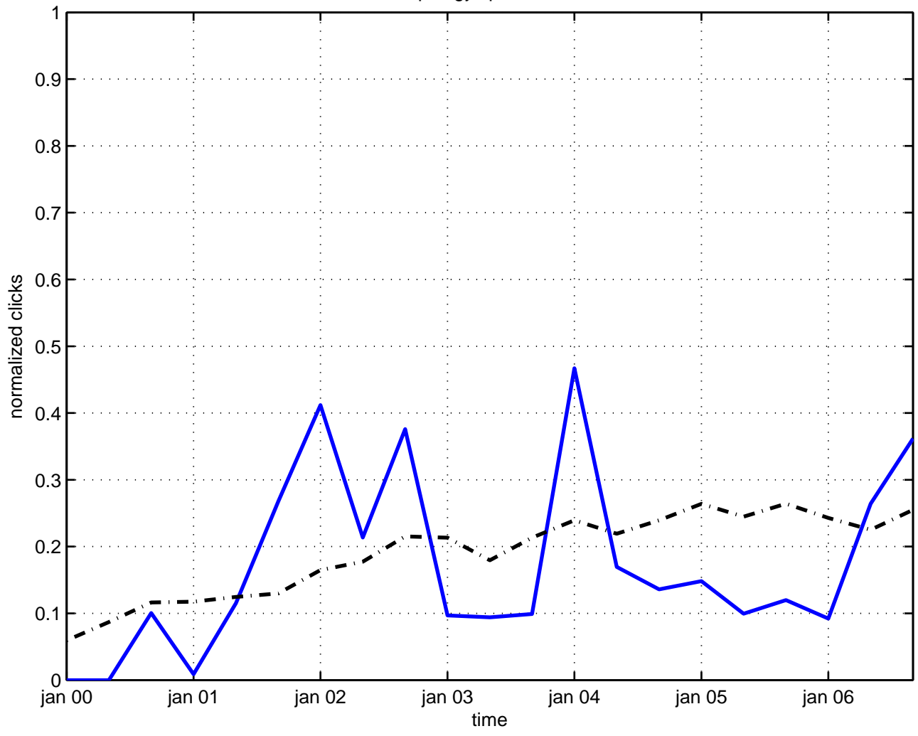
topology space-time
